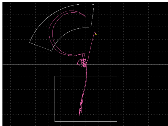
MIA mode configured to identify a repaired area (bottom signal) as opposed to a disbanded condition (top signal).
